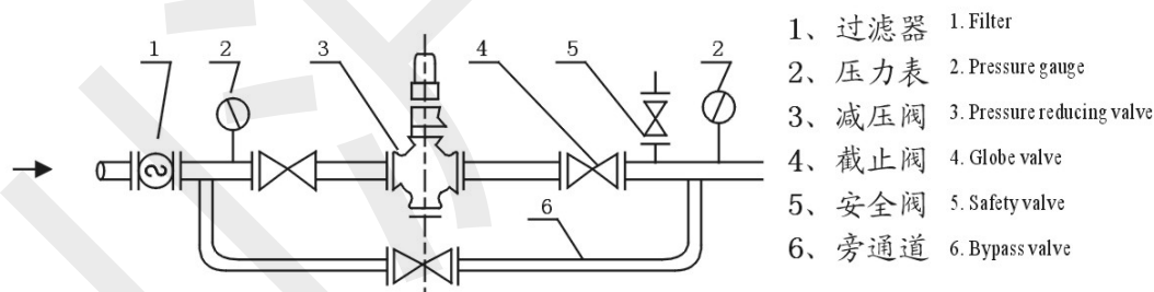
Installation Diagram
